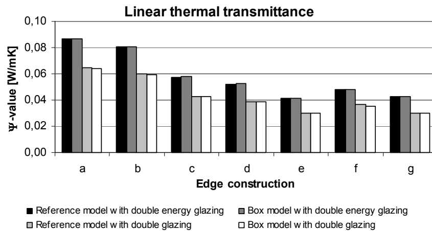
Figure A4.2: Linear thermal transmittance simulated for a wood/aluminium frame profile (Figure A4.1)
