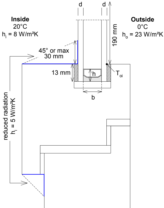
Figure 3: Sketch of the modified standard frame profile from “prEN ISO 10077-2” used to determine the equivalent thermal conductivity ( \lambda_k ) in the box-model.
