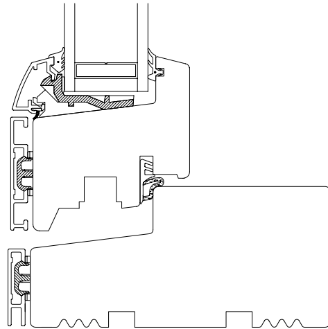
Figure A4.1: Sketch of wood/aluminium frame profile
