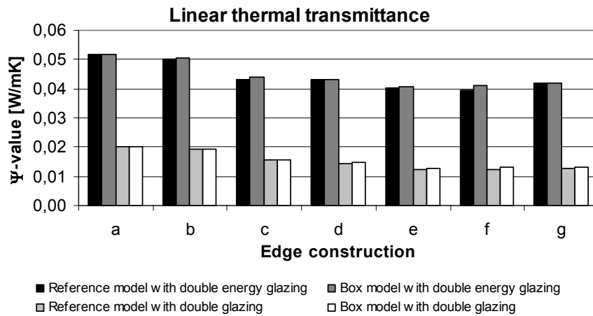
Figure A7.2: Linear thermal transmittance simulated for a wood/aluminium/pvc frame profile (Figure A7.1)
