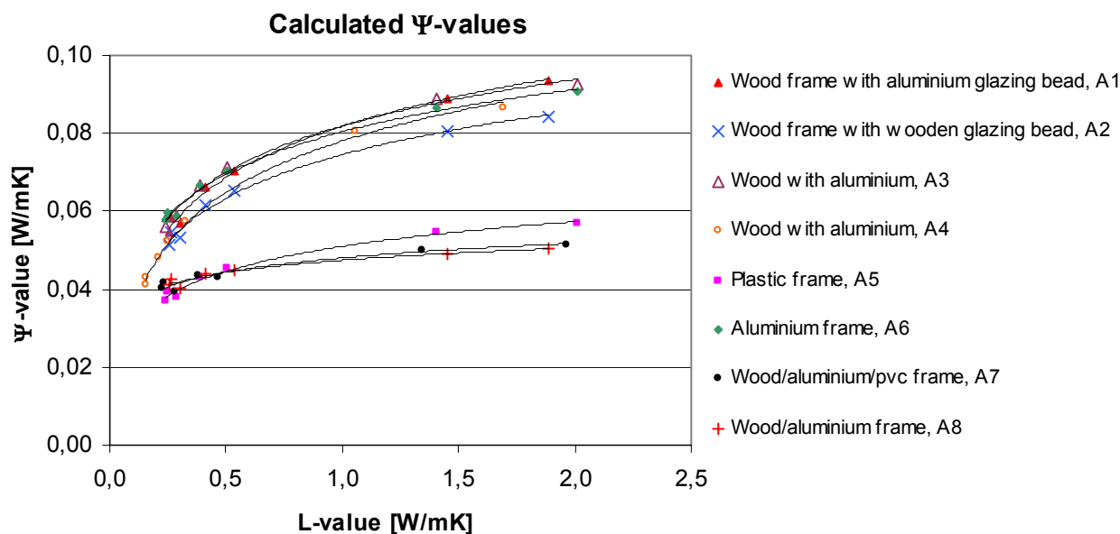
Figure 9: Calculated values of the linear thermal transmittance ( \Psi -value). The diagram provides results for eight different frames as a function of the thermal transmittance ( L ) of the edge construction valid for a double energy glazing with a thermal transmittance applicable to the centre of the glazing ( U_g ) of approximately 1.2 \text{ W/m}^2\text{K} . The frame profiles used in the calculations are shown in appendix A.
