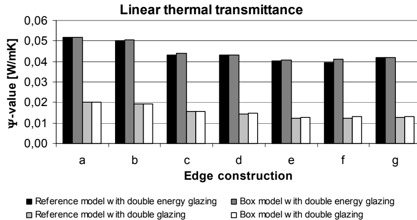
Figure 6: Linear thermal transmittance calculated for the reference model and the box model for an aluminium/wood/pvc frame profile (A7) with a double energy glazing and a double glazing.
