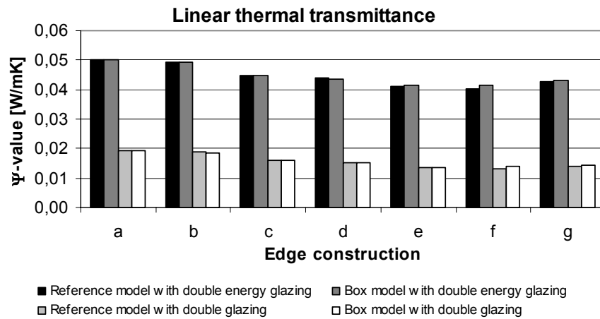
Figure A8.2: Linear thermal transmittance simulated for a wood/aluminium frame profile (Figure A8.1)
