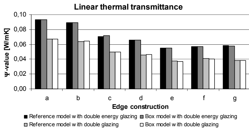
Figure A1.2: Linear thermal transmittance simulated for a wood frame profile with aluminium glazing bead (Figure A1.1)
