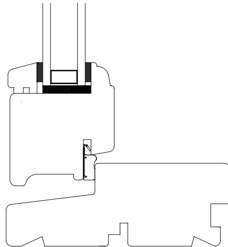
Figure A2.1: Sketch of wood frame profile with wooden glazing bead
