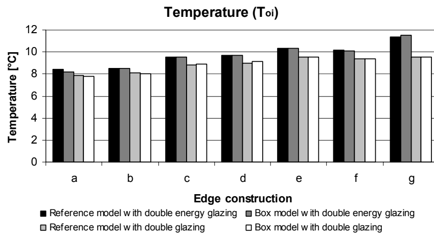
Figure A3.3: Temperature on the lower part of the inner glazing simulated for a wood/aluminium frame profile
