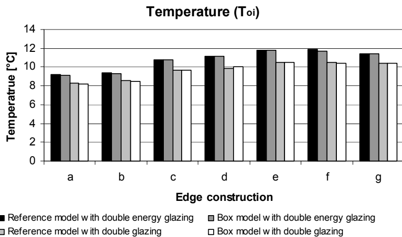
Figure A1.3: Temperature on the lower part of the inner glazing simulated for a wood frame profile with aluminium glazing bead
