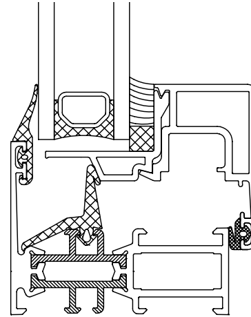
Figure A6.1: Sketch of aluminium frame profile
