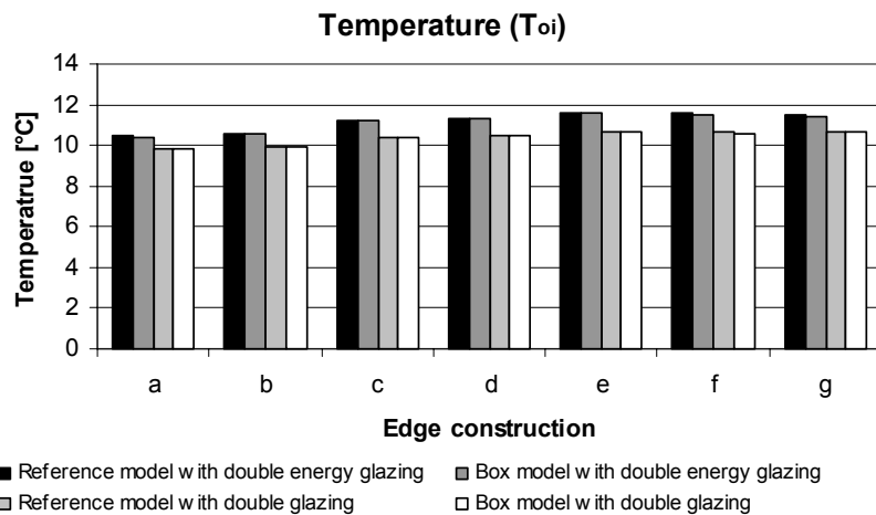
Figure A6.3: Temperature on the lower part of the inner glazing simulated for a aluminium frame profile
