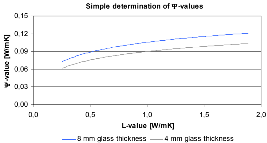
Figure 10: Diagram for simple determination of the linear thermal transmittance ( \Psi -value). The diagram uses the thermal transmittance ( L ) of the edge construction and the glass thickness as input and is valid for a double energy glazing with a thermal transmittance applicable to the centre of the glazing ( U_g ) of approximately 1.2 \text{ W/m}^2\text{K} .
