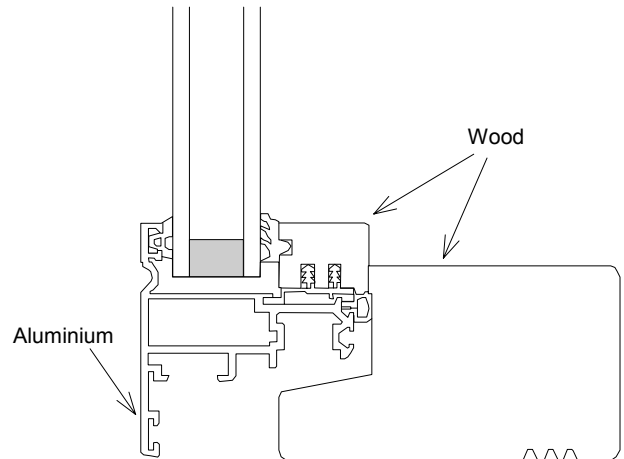
Figure A8.1: Sketch of wood/aluminium frame profile
