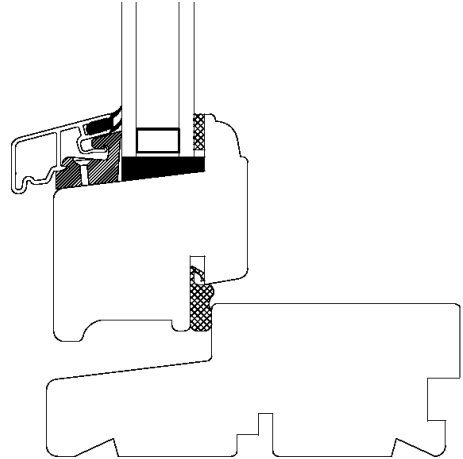
Figure A1.1: Sketch of wood frame profile with aluminium glazing bead
