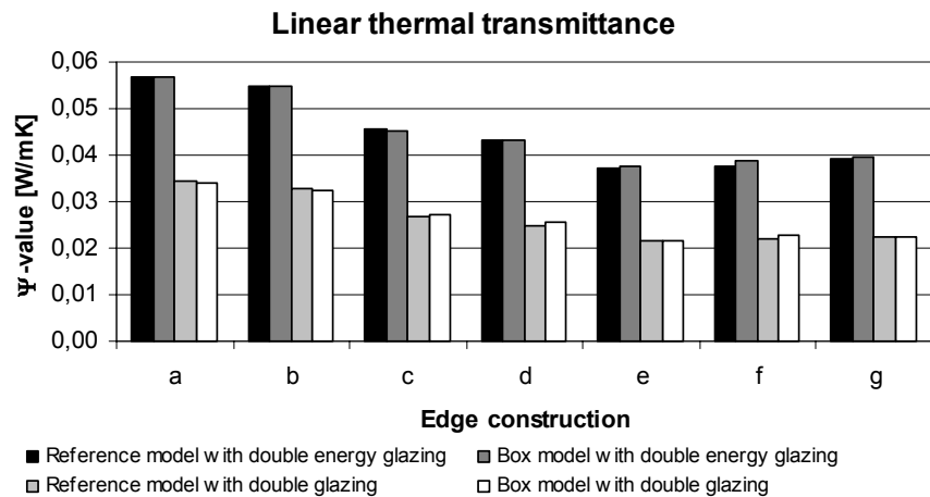
Figure A5.2: Linear thermal transmittance simulated for a plastic frame profile (Figure A5.1)
