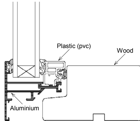
Figure A7.1: Sketch of wood/aluminium/pvc frame profile
