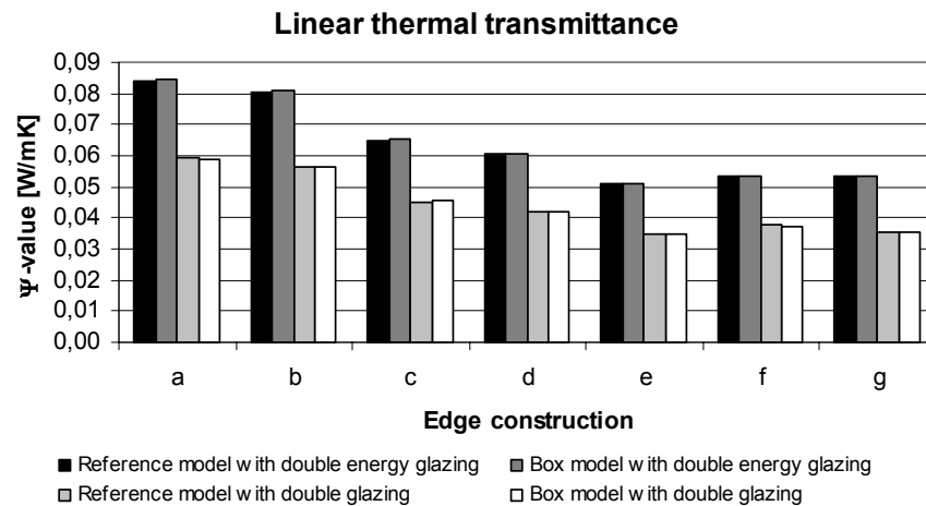
Figure A3.2: Linear thermal transmittance simulated for a wood/aluminium frame profile (Figure A3.1)
