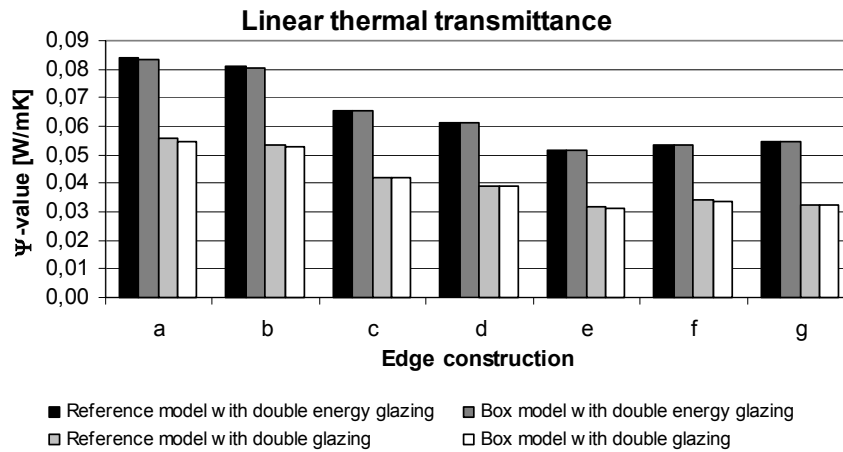
Figure A2.2: Linear thermal transmittance simulated for a wood frame profile with wooden glazing bead (Figure A2.1)
