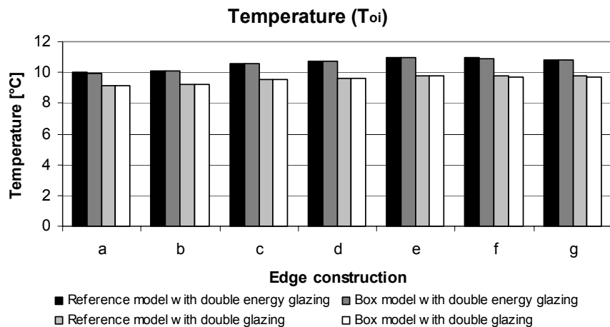
Figure A5.3: Temperature on the lower part of the inner glazing simulated for a plastic frame profile
