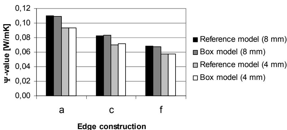
Figure 8: Variation of glass thickness from 4 mm to 8 mm in the wood frame profile with aluminium glazing bead (frame profile A1).
