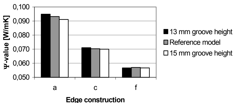
Figure 2: Influence of groove height in the wooden frame profile with aluminium glazing bead (A1).
