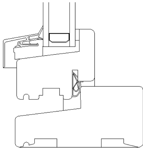
Figure A3.1: Sketch of wood/aluminium frame profile
