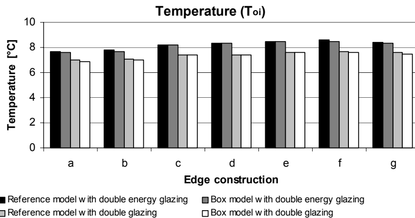
Figure 7: Temperature on the lower part of the inner glazing calculated for the reference model and the box model for an aluminium/wood/pvc frame profile (A7) with a double energy glazing and a double glazing.
