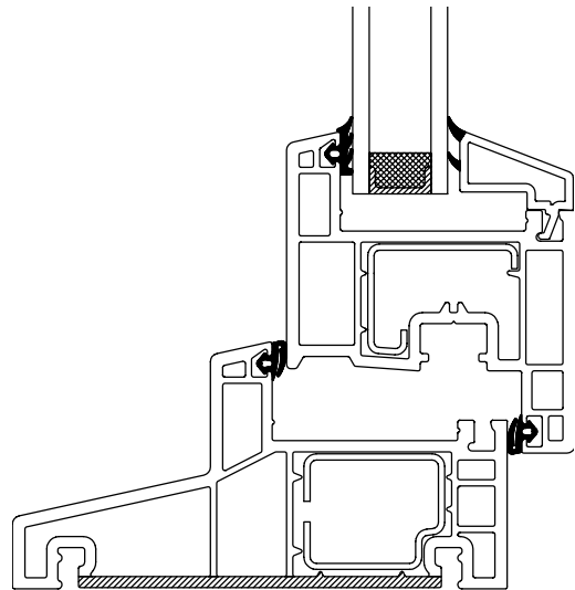
Figure A5.1: Sketch of plastic (pvc) frame profile
