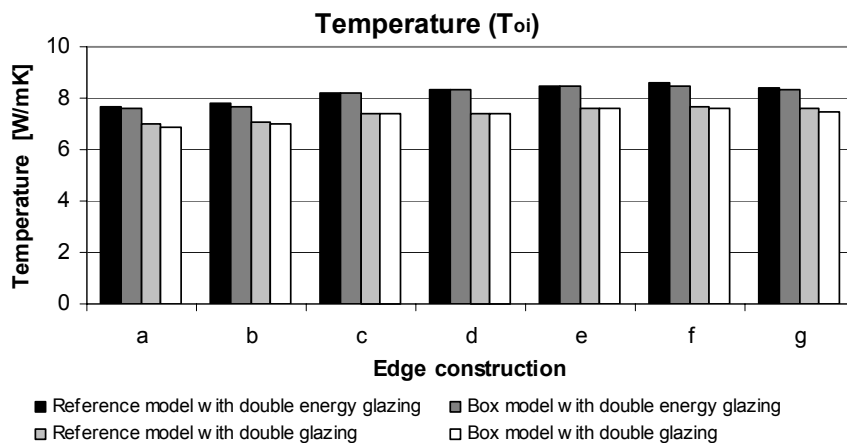
Figure A7.3: Temperature on the lower part of the inner glazing simulated for a wood/aluminium/pvc frame profile
