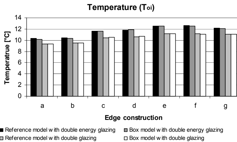
Figure A2.3: Temperature on the lower part of the inner glazing simulated for a wood frame profile with wooden glazing bead
