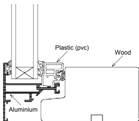
Figure 5: Sketch of the modelled frame profile made from aluminium, wood and pvc (frame profile A7).
