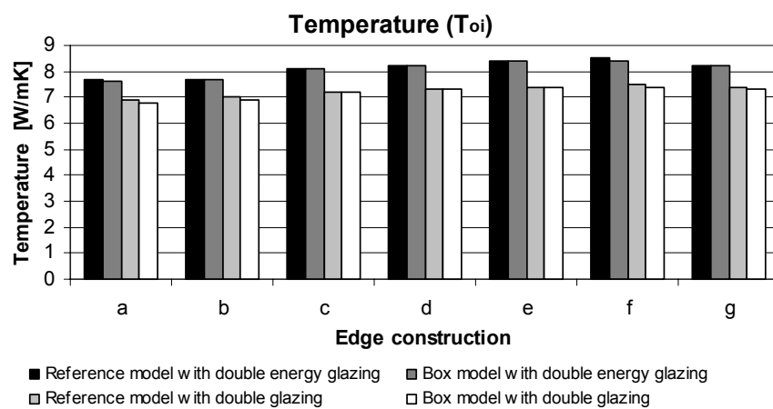
Figure A8.3: Temperature on the lower part of the inner glazing simulated for a wood/aluminium frame profile
