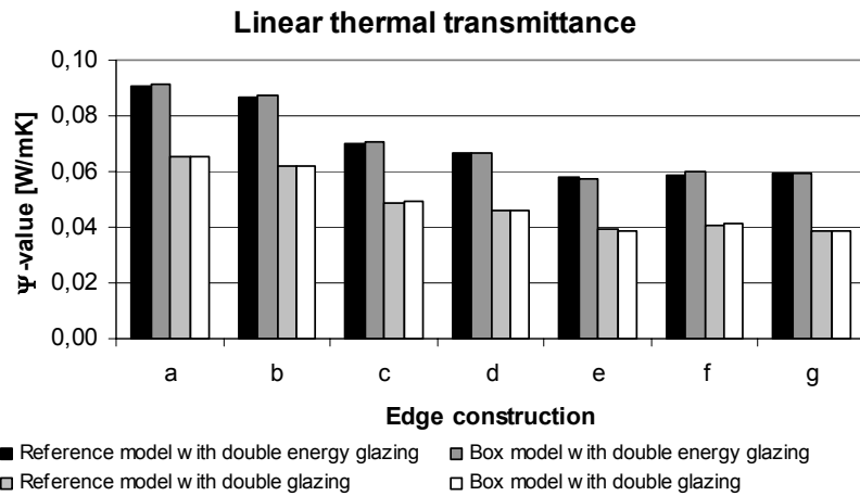
Figure A6.2: Linear thermal transmittance simulated for a aluminium frame profile (Figure A6.1)
