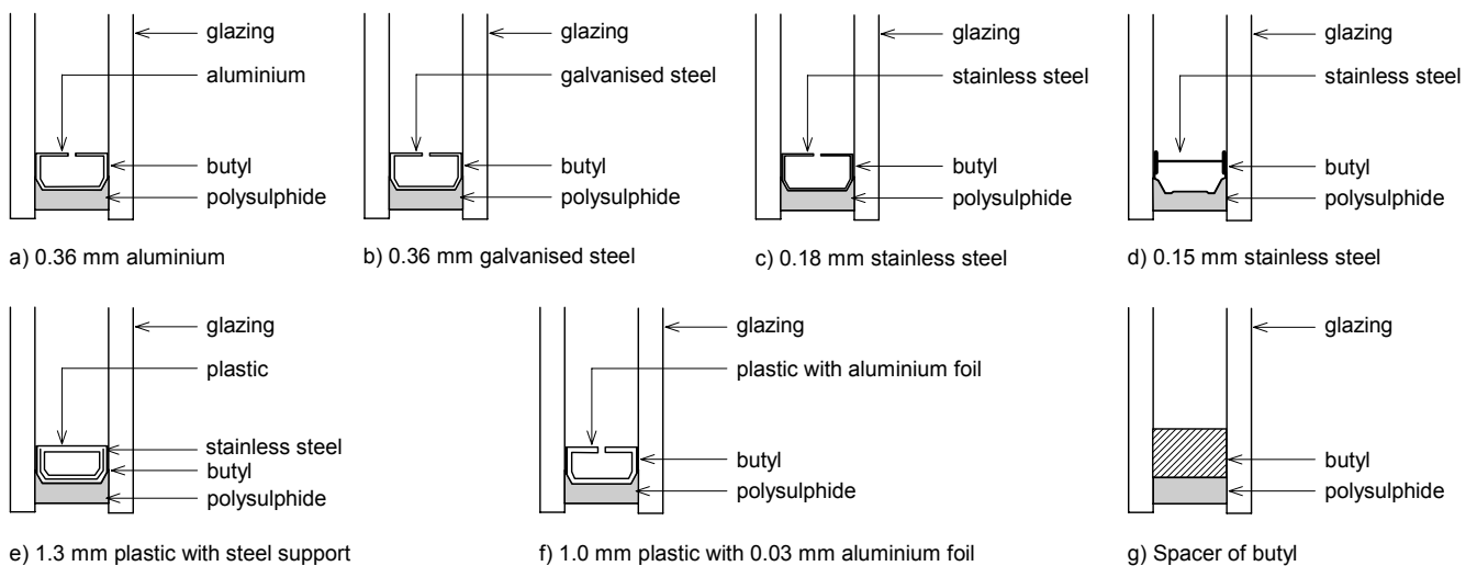
Figure 4: Sketch of the modelled edge constructions.
