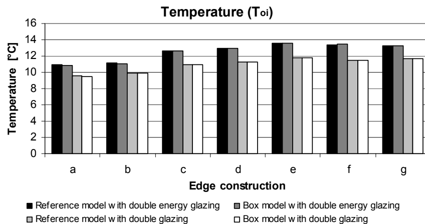
Figure A4.3: Temperature on the lower part of the inner glazing simulated for a wood/aluminium frame profile
